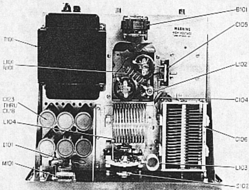
Fig. 4 - Top View of Chassis
